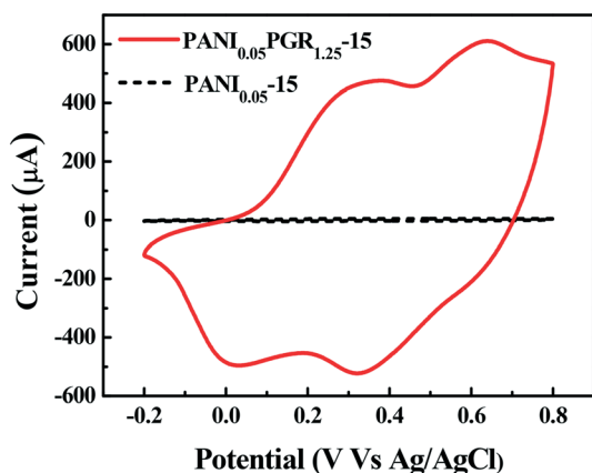
Fig. 3 CV curves of the PANI 0.05 -15 and PANI 0.05 PGR 1.25 -15 modified GCE at a scanning rate of 100 mV·s -1 in 0.1 M H 2 SO 4 .
