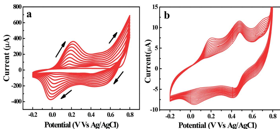
Fig. 2 CV curves of aniline electropolymerization on the PGR modified GCE (a) and the bare GCE (b) at a scanning rate of 100 mV·s -1 in 0.1 M H 2 SO 4 .
