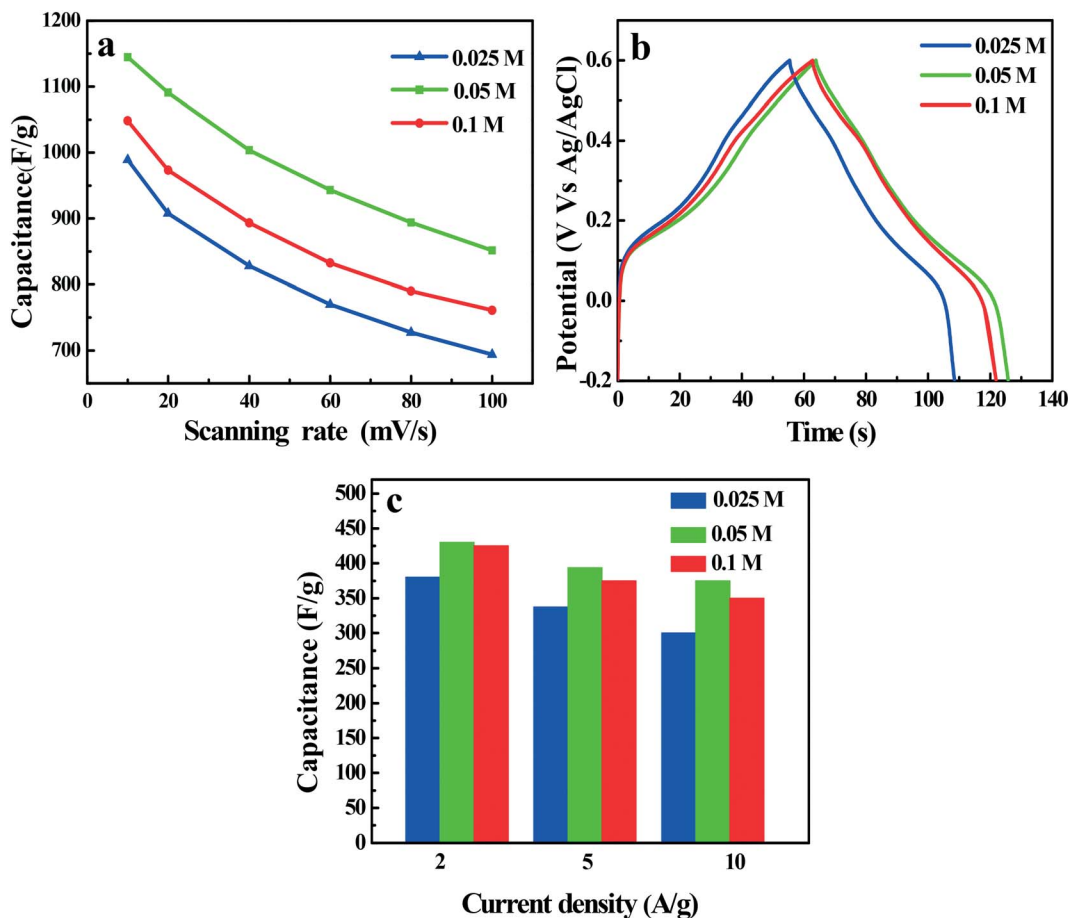
Fig. 5 (a) Specific capacitance of the PANI 0.025 PGR 1.25-15 , PANI 0.025 PGR 1.25-15 and PANI 0.1 PGR 1.25-15 modified GCE by CV curves at different scanning rates from 10, 20 40, 60, 80 to 100 mV·s -1 , (b) GCD curves of the PANI 0.025 PGR 1.25-15 , PANI 0.025 PGR 1.25-15 , PANI 0.1 PGR 1.25-15 modified GCE at 5 A·g -1 , (c) Specific capacitance of the PANI 0.025 PGR 1.25-15 , PANI 0.025 PGR 1.25-15 and PANI 0.1 PGR 1.25-15 modified GCE from GCD at different current density from 2, 5 to 10 A·g -1 .
