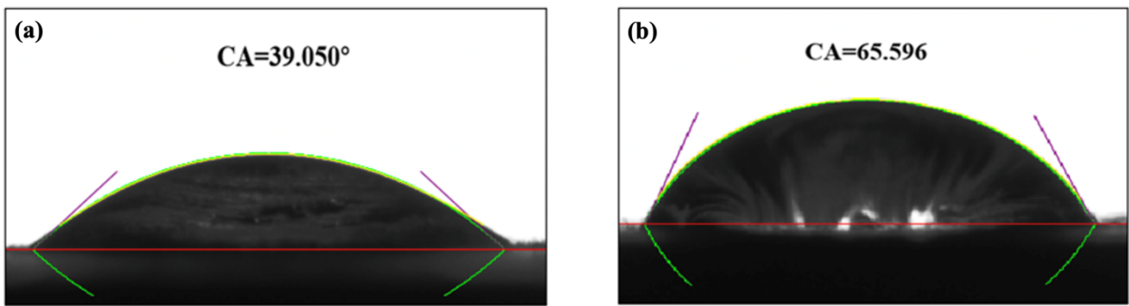
Fig. S2 Contact angle of (a) untreated wood and (b) PS/Ti 0.87 O 2 composite.
