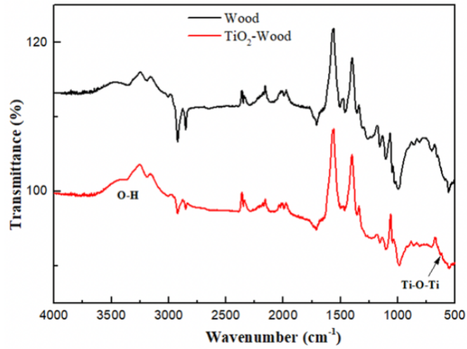
Fig. S1. FTIR spectrum of the natural wood and PS/Ti 0.87 O 2 composite.
