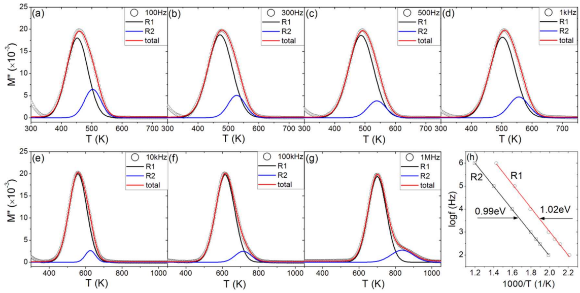
Figure S1. Two-relaxation fittings for the electric modulus spectra of CSO (a-g) and the resultant Arrhenius plots of the relaxations (h).
