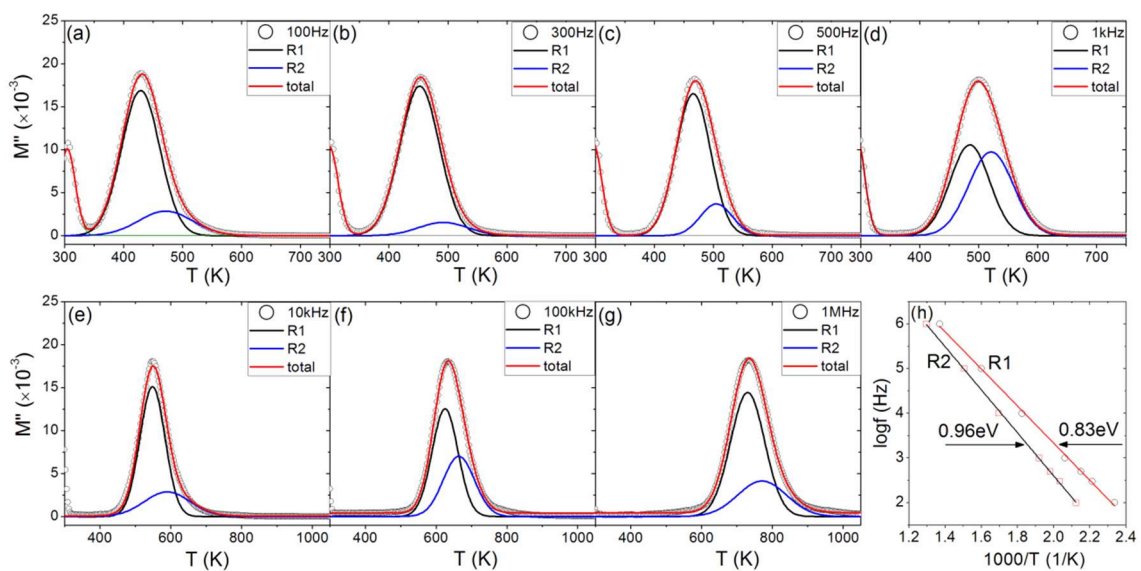
Figure S2. Two-relaxation fittings for the electric modulus spectra of CNO (a-g) and the resultant Arrhenius plots of the relaxations (h).
