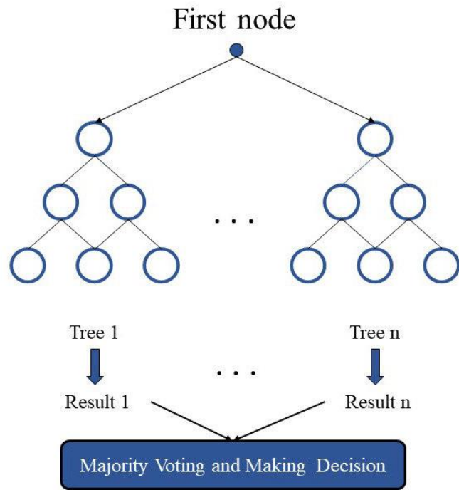
Fig. S2. Schematic representation of the random forest [31]
